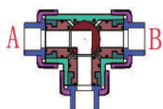
L - TYPE FLOW: CA / CB
